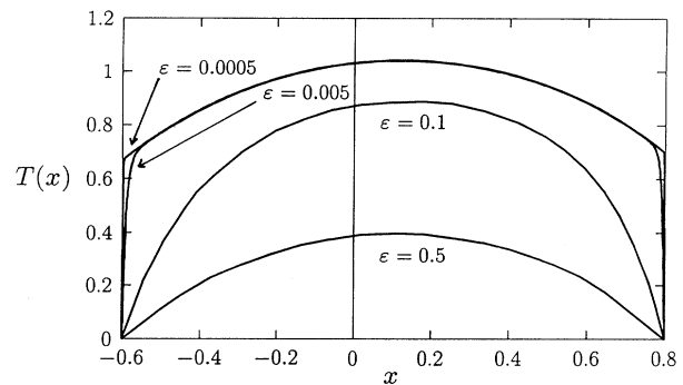
FIG. 7. MFPT T(x) for the diffusively perturbed system (59) and (60) and for the second class of intervals, A = -0.6 , B = 0.8 , for several values of the perturbation parameter \varepsilon and fixed D = a = \nu = 1 .
